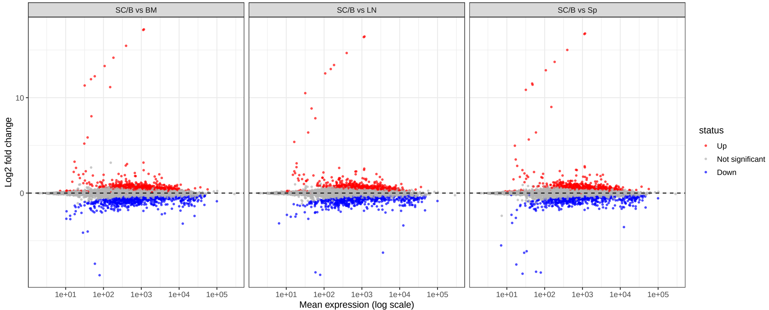
MA plot: Expression changes in SC/B vs SP, LN, and BM
